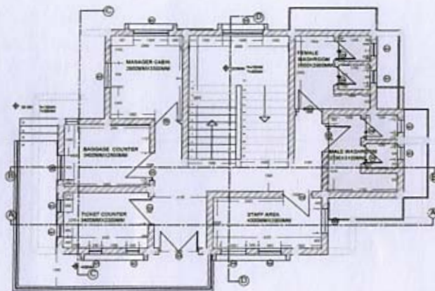
GROUND FLOOR PLAN SCALE : 1/50
